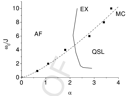
Fig. 3. The phase boundary AF-QSL calculated by MC and the expansion in terms of small parameter (EX) [8].
