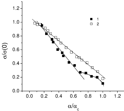
Fig. 1. The magnetic moment per site as a function of the spin-phonon coupling for \omega_0 = J (1), \omega_0 = 6J (2).
