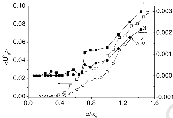
Fig. 2. Mean-square vibration \langle U^2 \rangle vs. spin-phonon coupling at \omega_0 = J (2,4), \omega_0 = 6J (1,3) along [10] (1,2, \beta = x ), [01] (3,4, \beta = y ) directions.
